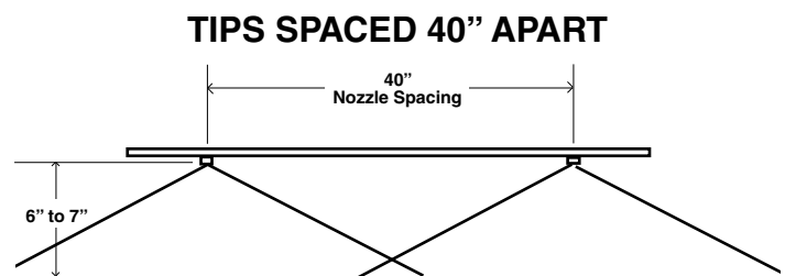
Flat Uniform Sprayer Pattern
